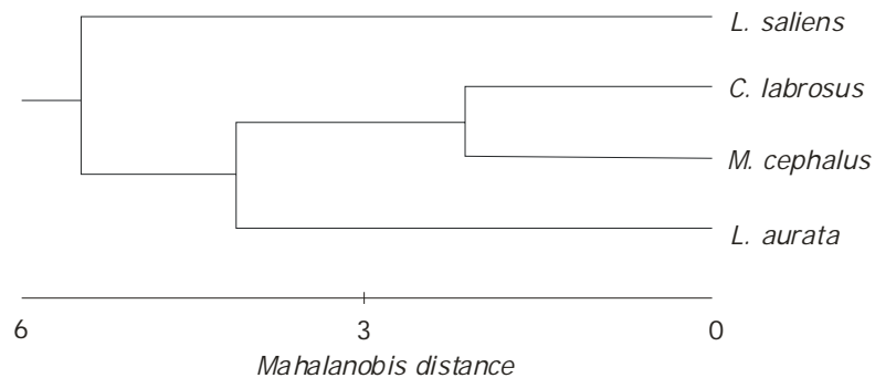
Figure 4. UPGMA cluster analysis based on the Mahalanobis distance between the species centroids.
