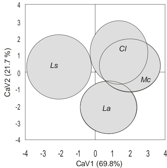
Figure 3. Discriminant analysis plot where the 8 morphometric variables were used. Ls : Liza saliens , La : Liza aurata , Cl : Chelon labrosus , Mc : Mugil cephalus . Ellipses include 95 % of the specimens.
