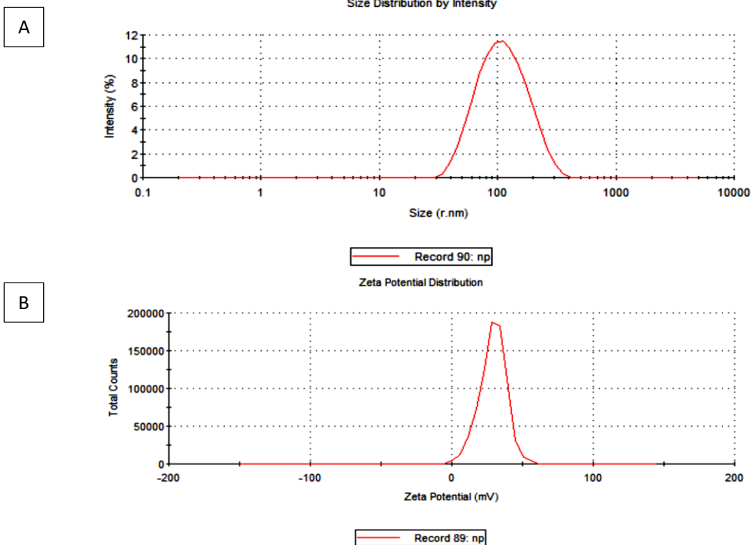
Figure 1. Particle size (A) and zeta potential distribution (B) of chitosan nanoparticles.
