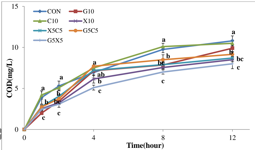
Figure 2. Water COD changes after the addition of diets (CON, G 10 , C 10 , X 10 , X 5 C 5 , G 5 C 5 and G 5 X 5 ) for 12 hrs into the water
